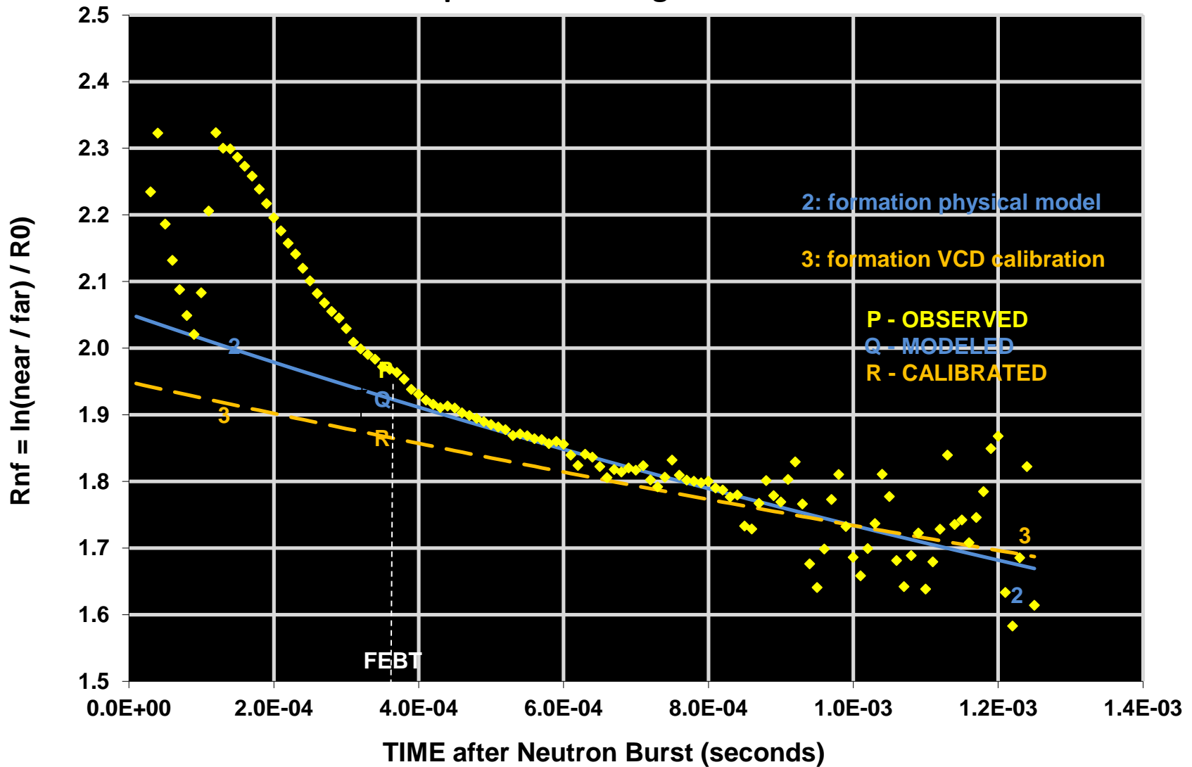
FIGURE TWO: Rnf versus TIME in 100% FW - Calibration and Borehole Compensation Using van Cittert Deconvolution
