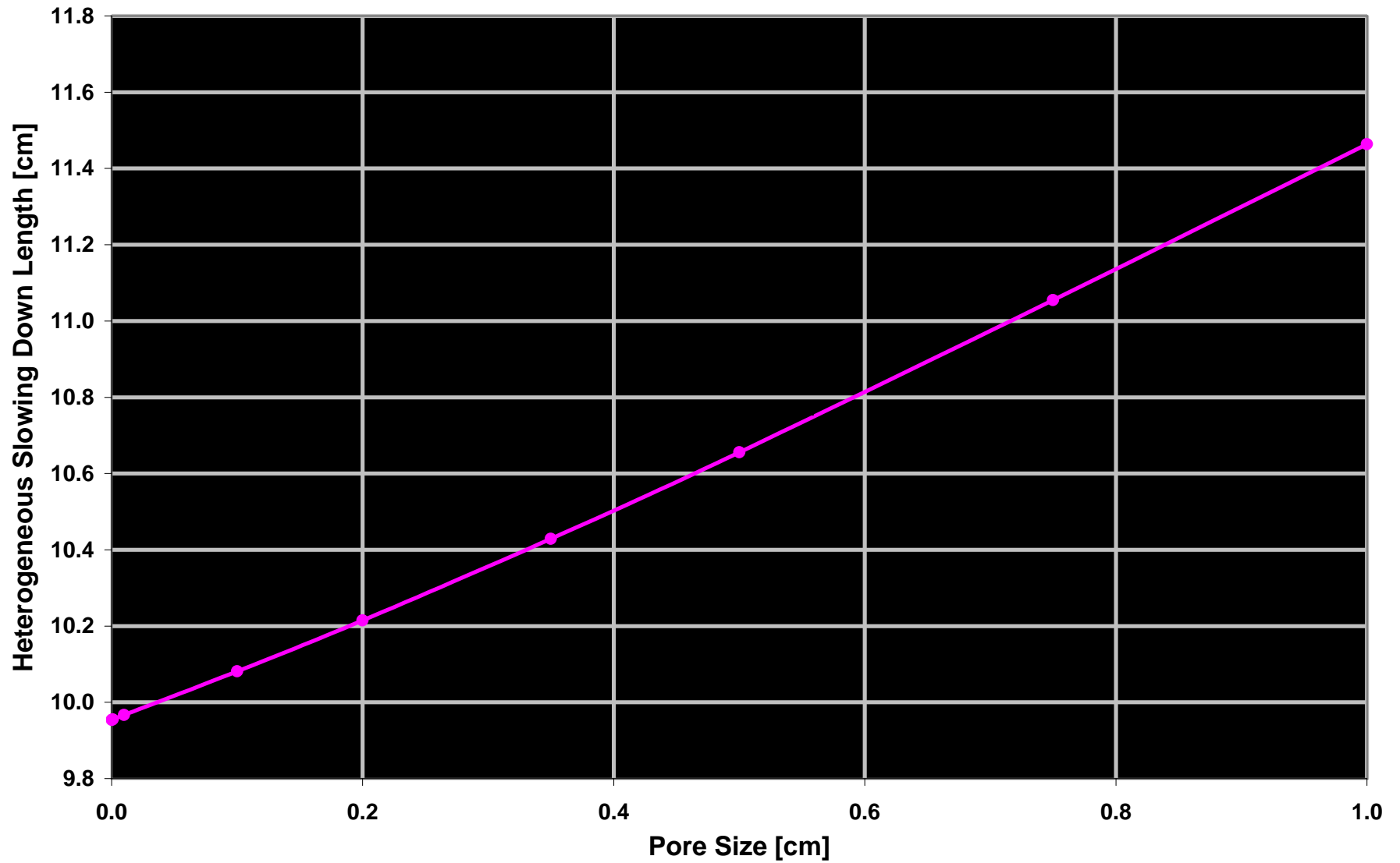
Heterogeneous Slowing Down Length versus Pore Size for a 20% Oil Saturated Dolomite
