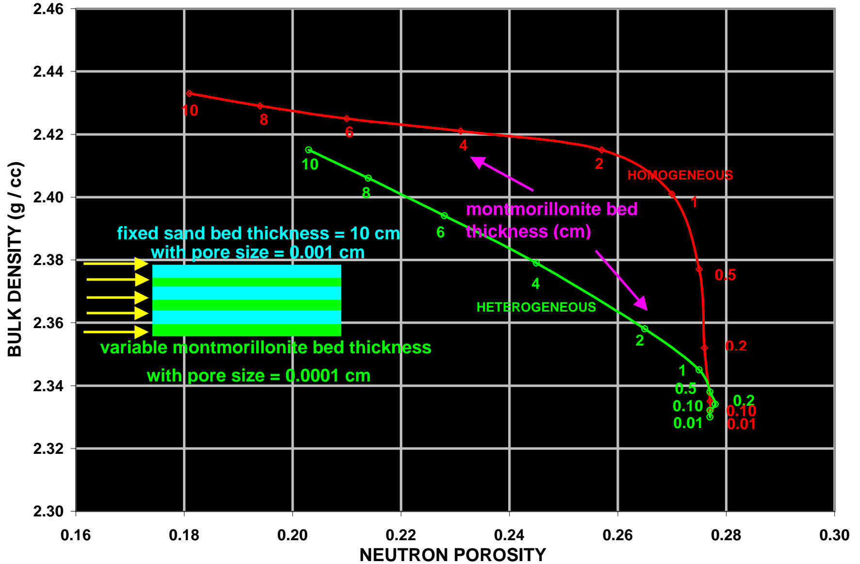
BULK DENSITY versus NEUTRON POROSITY
